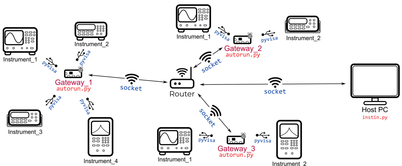
FIGURE 1. An illustrated scheme of the proposed wireless instrumentation control system. The host PC is connected to the same WiFi network than the Raspberry-based gateways. Each gateway can be connected up to four instruments using their USB control ports. The python packages used to manage the communication protocols are shown in blue, and the developed control libraries (instin.py for the host PC and autorun.py for the gateways) are shown in red.
